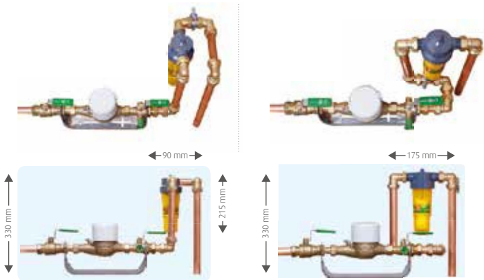
NoCalc CombiCompact
